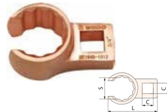
Crow Foot Box End
