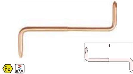
Phillips Offset Screwdriver
